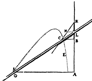
Descartes' drawing of the hyperbola referred to his co-ordinates
