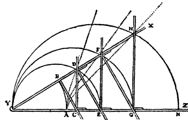
Descartes' curves drawn by his hinged instrument
