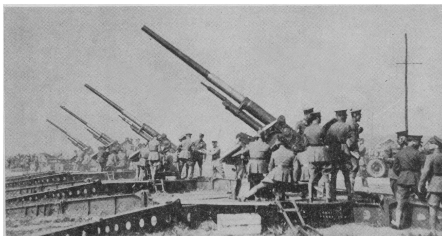
NEW MOBILE GUN mount, as used with a battery of anti-aircraft guns at the Aberdeen Proving Grounds, in Maryland. Note the folding spider-like legs, projecting from each corner, which stabilize the mount
