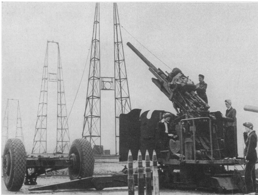
BULLETS CLOCKED —The range velocity towers record the speed of the shell from this big 90-mm gun through space. The shell is magnetized so that when it passes the hoops it sets up an electric current which is automatically recorded and timed.
