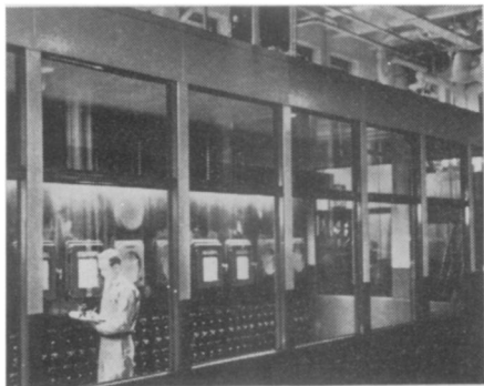
Reading Micromax Recorders in Penicillin Plant of Charles Pfizer & Co.
