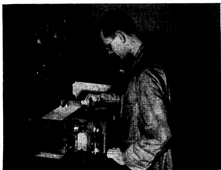
Checking pH With L&N Indicator
