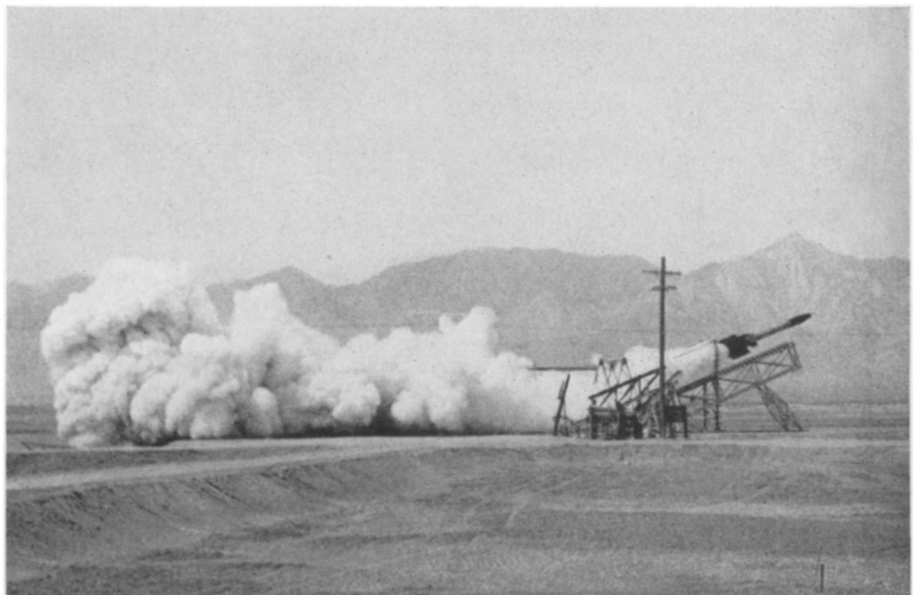
SUCCESSFUL FLIGHT TRIAL —This shows the largest supersonic ram-jet engine ever flown leaving the launching rack. The ram-jet must first be boosted to high speed by a rocket, which then drops off, leaving it to continue under its own power.
