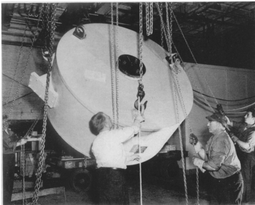
CHAMBER FOR ATOM-SMASHING —This steel tank houses the accelerating chamber of the 300,000,000-electron volt synchrotron being built in the General Electric Research laboratory.
