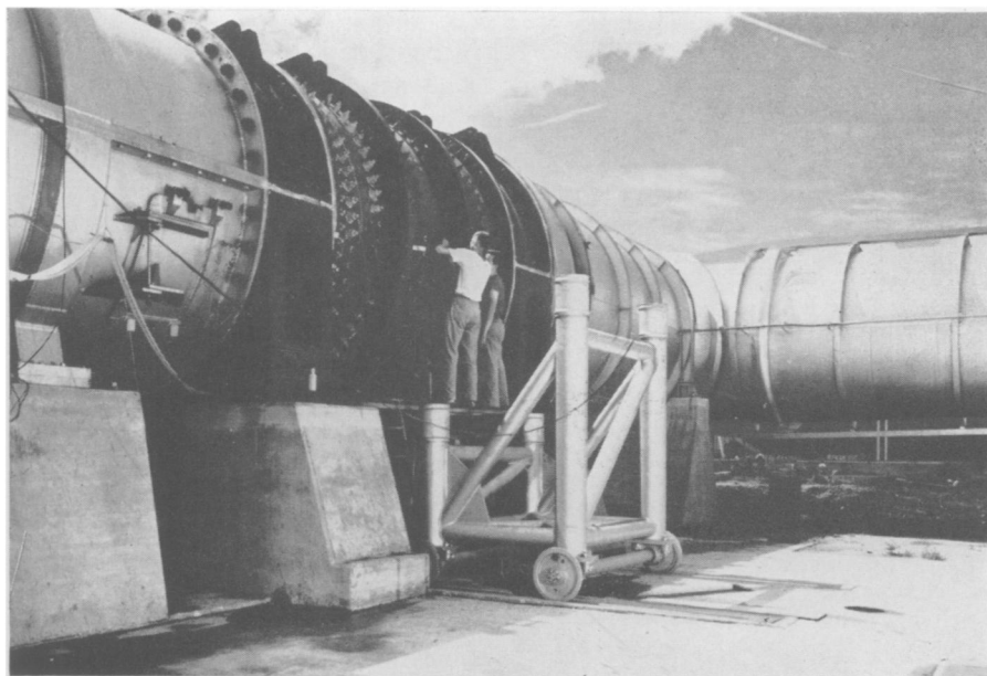
NEW SUPERSONIC TUNNEL —Most important single element of the huge tunnel is this 870,000 cfm axial flow compressor.
