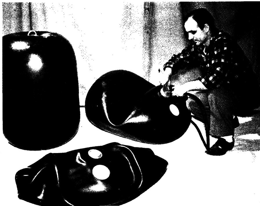
RUBBER SHIPPING DRUM —The new 55-gallon rubber drum suitable for shipping liquids is shown in three stages. At left is a filled drum, in the foreground, a collapsed drum, and at the right a drum being filled, for which no vent is needed. Since the drums collapse when empty, valuable shipping space can be saved when they are being returned.
