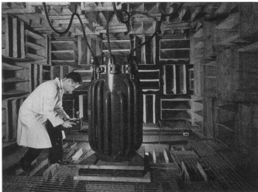
ANECHOIC LABORATORY —Quieter fluorescent lights, transformers and other electrical equipment are expected to result from studies now being made in this specially designed room, center of operations in the new Westinghouse acoustics laboratory. Charles H. Smith, engineer, is measuring the slight hum of a transformer.
