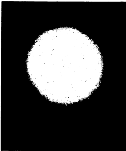
X-RAY "FOOTPRINT" —Electrons from the synchrotron at the California Institute of Technology, accelerated to energies of 460 million electron volts, bombarded a lead plate, producing the world's most energetic X-rays and giving this "footprint" on film.
