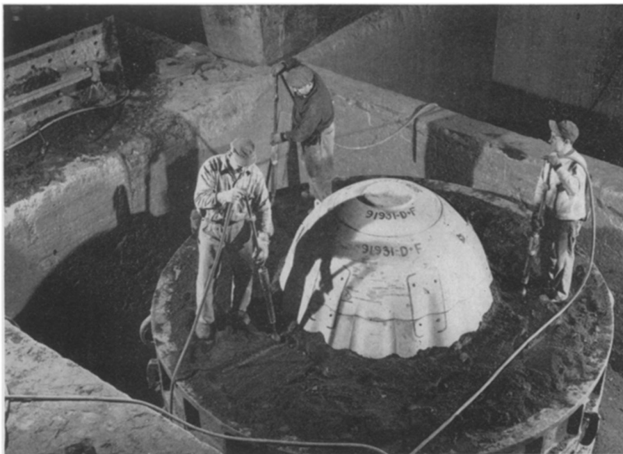
MAKING SLAG HOLDERS —One of the steps in making the containers that hold the fiery tons of molten slag dumped from open hearth and blast furnaces is shown here. Workmen of the Mackintosh-Hemphill Co. are making sure the silica facing sand covers all pattern surfaces, inside and outside.
