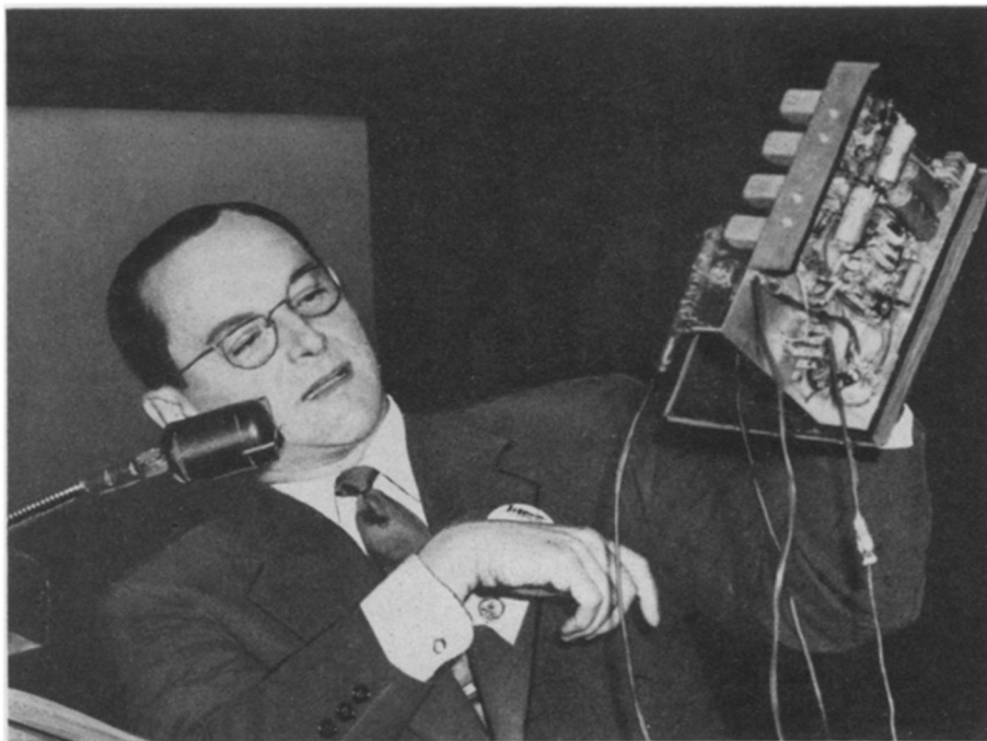
TRANSISTOR RECEIVER —Experimental model of a transistor receiver is demonstrated by Dorman D. Israel, executive vice-president of Emerson Radio and Phonograph Corporation, who predicts that in less than three years mass production of "shirt-pocket" radios will make this prototype a "grand-daddy." Transistors, made with a tiny disk of germanium, can replace vacuum tubes for many purposes.
