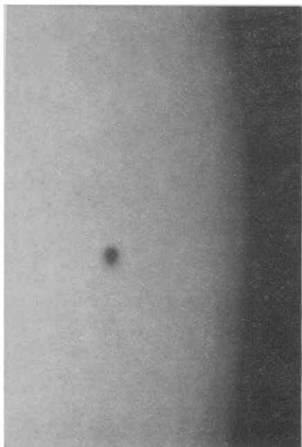
MERCURY DURING TRANSIT— Taken at 12:25 p.m. EST on Nov. 14 at the U. S. Naval Observatory in Washington, this picture shows the planet Mercury during its most recent transit of the sun, as it appeared by telescope. This rare astronomical event, when Mercury appears as a black dot on the sun, occurs only 13 or 14 times a century. (See SNL, Nov. 7, p. 298.)
