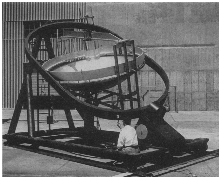
SOLAR FURNACE —Rays from the sun are collected by an aluminum mirror with a 120-inch diameter and reflected to a focal point five-sixteenths of an inch in diameter in this large Convair solar furnace. With ideal sky conditions, the furnace can develop a temperature of 8500 degrees Fahrenheit.
