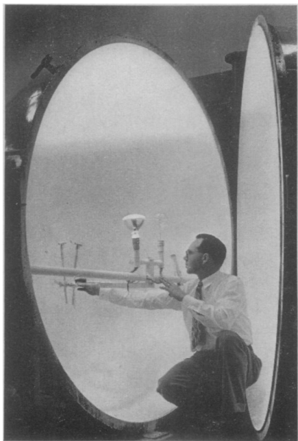
"INTEGRATING SPHERE" — To measure the total amount of light coming from a light source, this sphere has been built at the University of California. Final adjustments to calibrate the test lamp on the left are being made.
