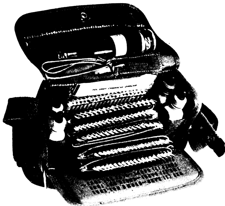
GAS DETECTOR KIT —Fast killing nerve gases and other war gases in the air have their presence shown by color reactions with the specially prepared silica gel in these clips.
