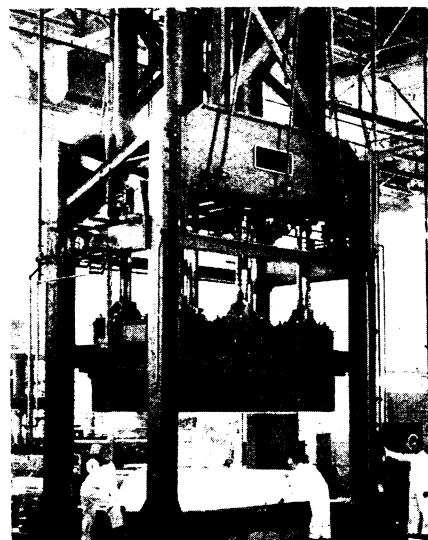
BOAT PRESS —Workmen prepare to remove a bull from this 700-ton press, believed to be the largest of its kind. It was designed for forming one-piece plastic hulls for outboard motor boats. This machine is one of five of its kind that has been installed in Goodyear Aircraft Corporation's plant.
