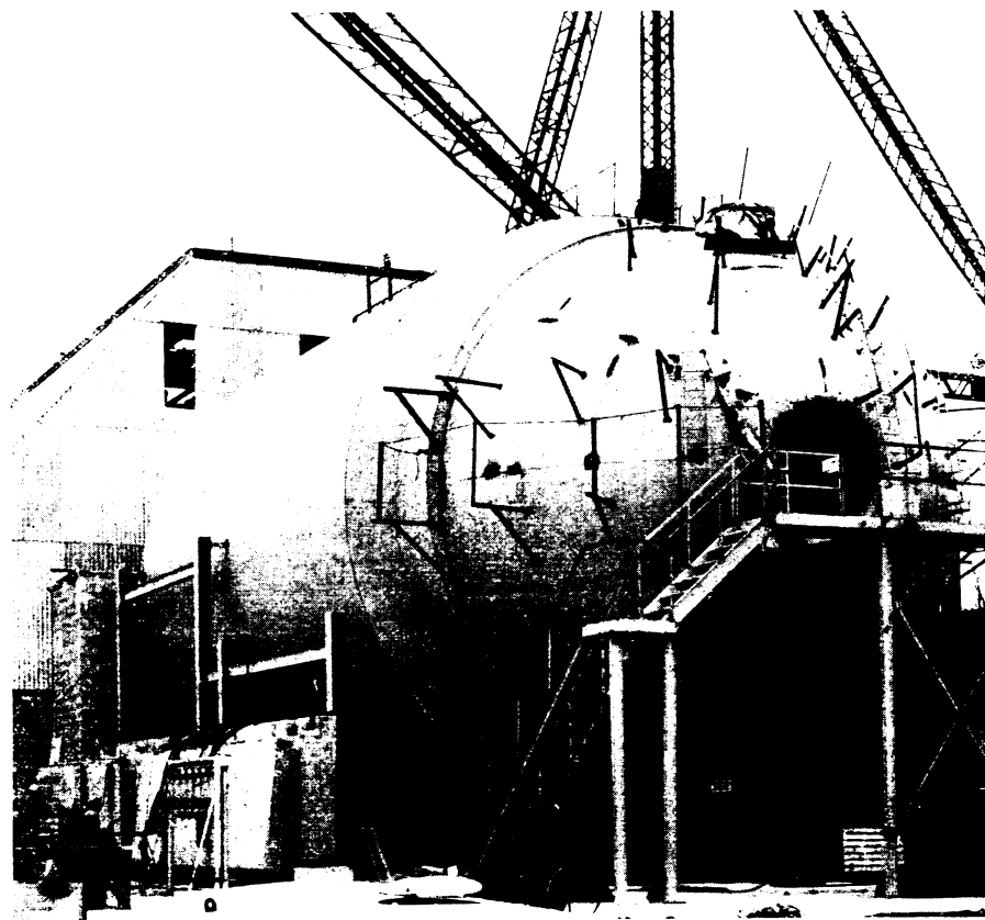
TRITON—The submarine hull section shown nearing completion at West Milton, N. Y., will house the prototype of the nuclear propulsion plant for the U. S. Navy's submarine, Triton. Described as the largest underwater craft ever built, it will be powered by two pressurized water reactors and will be the first such plant ever developed for submarine propulsion. Both the prototype and actual nuclear propulsion plant are being designed and developed at the General Electric Company's Knolls Atomic Power Laboratory.
