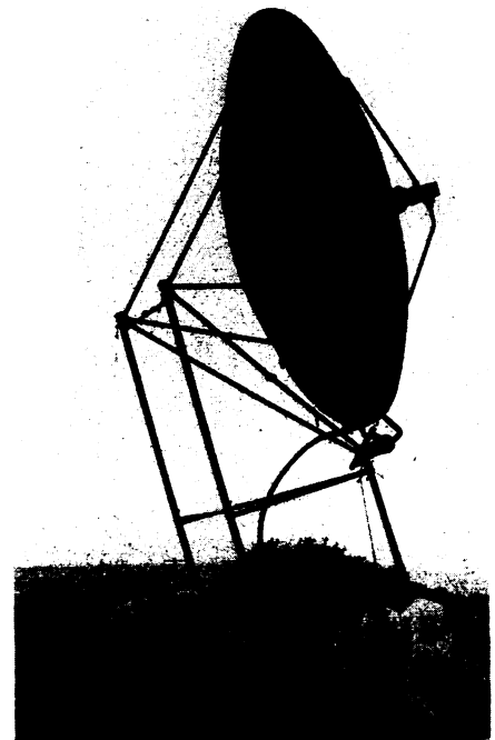
PORTABLE ANTENNA —This air-inflated antenna, part of the Collins UHF transhorizon terminal developed for the U. S. Army Signal Corps, may be easily erected or dismantled. Disassembled, the complete structure can be stored in a space approximately three feet by two feet by seven and a half feet.
