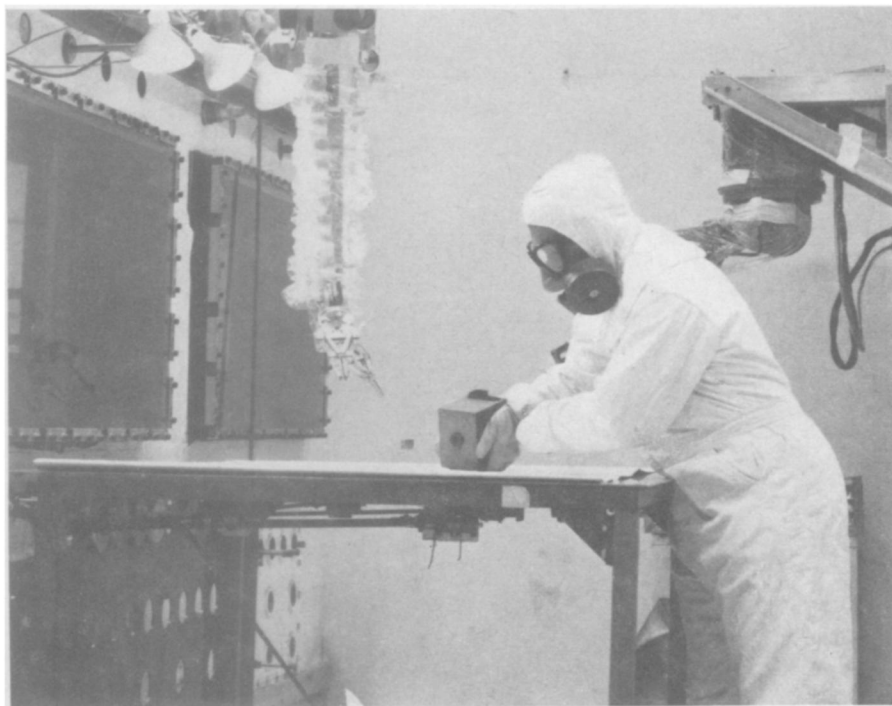
ATOMIC-AGE-CAMERA —An especially designed pin-hole camera, weighing 29 pounds, made from lead and uranium, is used for seeing into areas too "hot" for other detection devices. It carries two types of film: one for conventional light negatives and the other, an X-ray film, for recording atomic radiation. Designed by General Electric engineer John Payne, it is in use at the Knolls Atomic Power Laboratory, Schenectady, N. Y.
