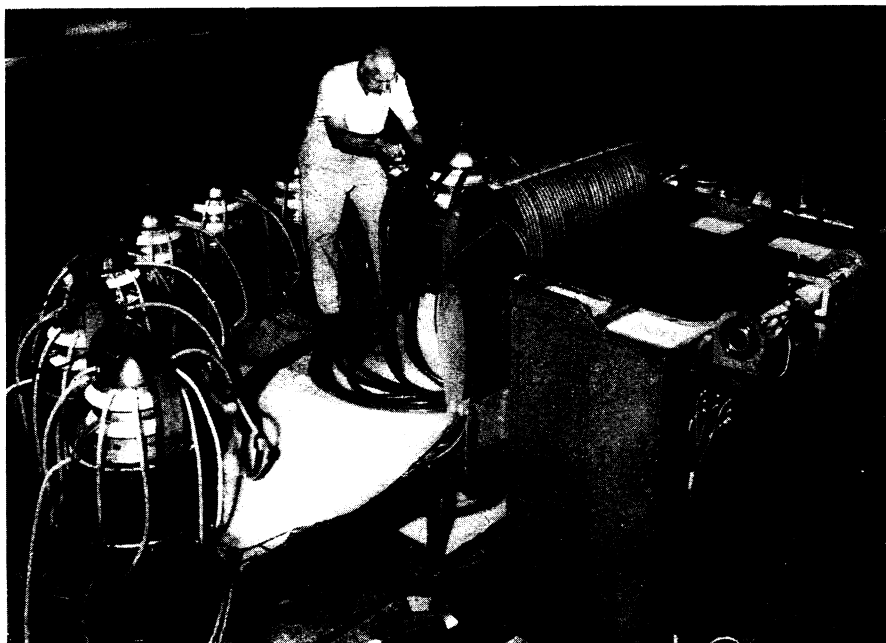
SCYLLA —Prof. William C. Elmore of Swarthmore College, a consultant to the Los Alamos Scientific Laboratory for the past year, makes final adjustments on the fusion device Scylla. The semicircular bank of capacitors is charged to 80 kilovolts and then discharged around the tube shown at the right of the photograph.
