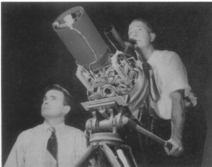
TRACKING TUMBLING —A new two-foot-long device, developed by the Raytheon Company, is demonstrated by engineers Andre Krutchkoff, left, and Wesley Haywood, who are tracking Echo I. The instrument was unveiled at Jupiter, Fla., during a meeting of tracking station experts of the Smithsonian Astrophysical Observatory's world-wide tracking network.
