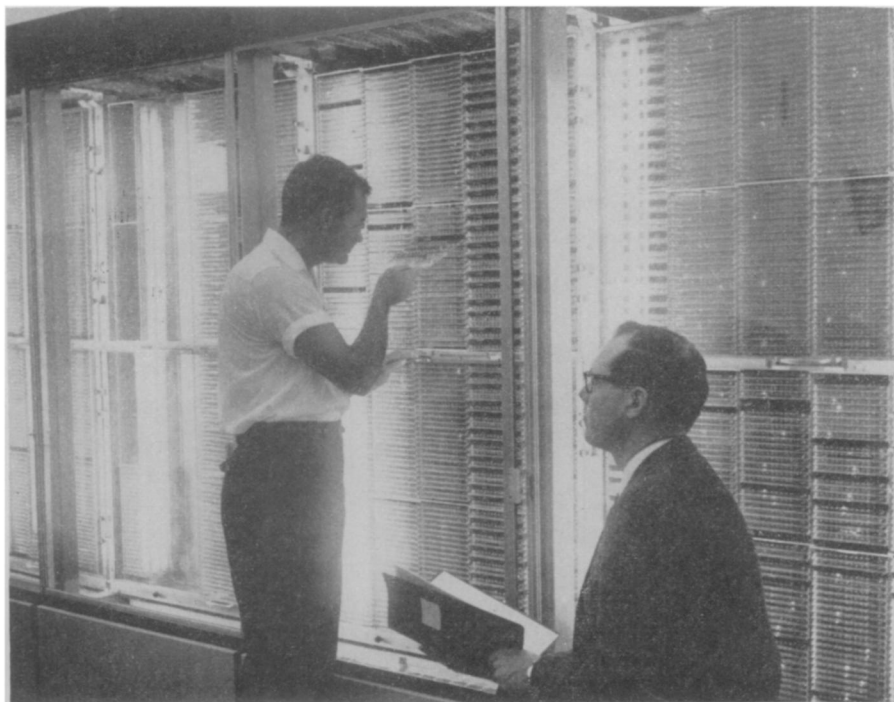
NEON TELEPHONE NETWORK —Telephone voices are carried through neon gas tubes that make up the "switching network" of an electronic central office developed by Bell Telephone Laboratories. The tubes are used to connect one telephone with another, a task that was earlier performed by electro-mechanical relays.
