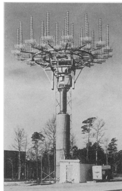
END-FIRE ANTENNA —will record telemetry from rockets tested at NASA's space flight station, Wallops Island, Va. It was built by General Bronze Corp., Garden City, N. Y.
