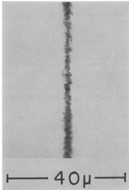
COSMIC RAY PATH —A microscopic photo shows the trail left by a cosmic ray through the interior of one of the silver chloride crystals developed by Dr. Lawrence M. Slifkin of the University of North Carolina department of physics. The trail has been made visible by a special process. The actual width of the trail shown is no more than one-tenthousandth of an inch.
