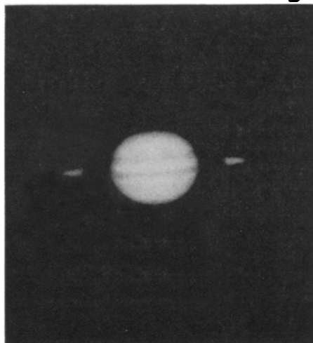
Naval Observatory
