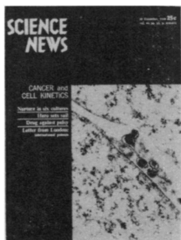
Electron microscope shows leukemia viruses in mouse tissue. Clearly recognizable only when they are outside a cell, the virus, center, looks like a tennis racket. p. 626 (Photo: Charles Pfizer & Co., Inc.)
