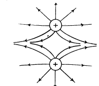
ELECTROSTATICS
