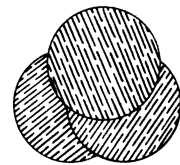
LIQUID CRYSTALS
