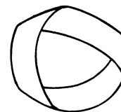
TOPOLOGY
