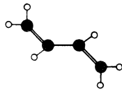
CHEMICAL MODELS
