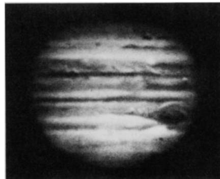
Water vapor is a first on Jupiter.
