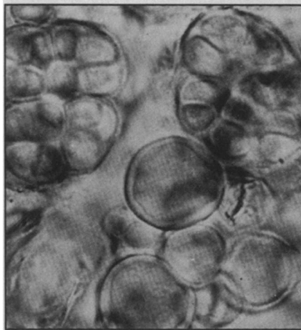
Pleurocapsalean fossils (top), compared to modern pleurocapsalean algae.
