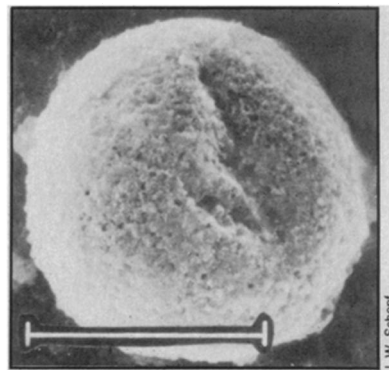
Schopf and late Precambrian microfossil from Bitter Springs formation, Australia.
