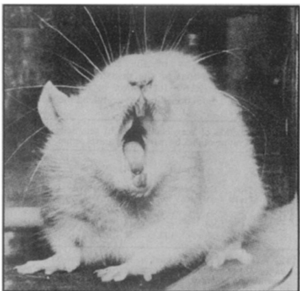
Physostigmine-induced yawning in a rat.
