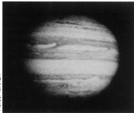
Jupiter: Germane to turbulence.
