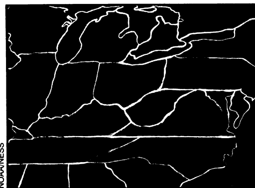
February 1978 (bottom) snow cover was 1.9 \times 10^6 km 2 more than the 10-year average. Jan. 23, 1978, GEOS-2 image shows midwest, southern and eastern U.S. snow cover.
