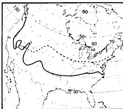
February 1978 (bottom) snow cover was 1.9 \times 10^6 km 2 more than the 10-year average. Jan. 23, 1978, GEOS-2 image shows midwest, southern and eastern U.S. snow cover.
