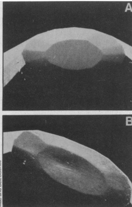
We have ways of making you yield. The flat face of a diamond anvil flowed into a permanent concave shape under 1.7 megabar pressure.
