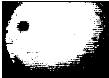
Time-lapse photomicrograph taken through a diamond window shows the crystalline form of hydrogen at 57 kilobars. Mao, Bell/SCIENCE
