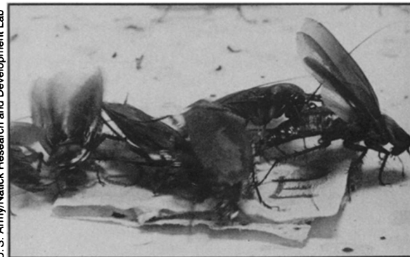
Natural female sex pheromone on a piece of filter paper excites male cockroaches.
