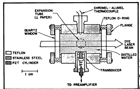
Schematic of Rydberg maser.
