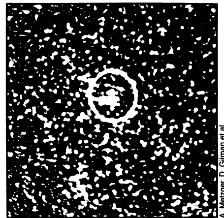
Jupiter by X-ray in HEAO-2 image.
