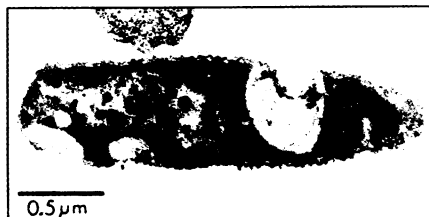
The upper electron micrograph shows an untreated Synechococcus blue-green alga. The lower micrograph shows the same cell after exposure to Scytonema extract.
