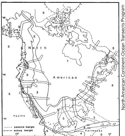
Map of North America shows the most ancient part of the land mass (1), parts of that mass deformed in the last 600 million years. (2), ancient displaced pieces of land (3), land fragments in transit (4), and oceanic crust (5). Geometric-shaped swaths indicate study areas that transect the ocean-continent margin.
