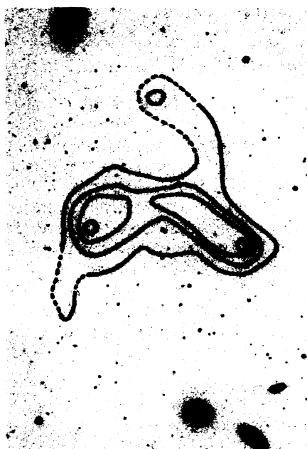
A map of radio emissions from neutral hydrogen in the cloud. Galaxies are in the upper left and lower right.
