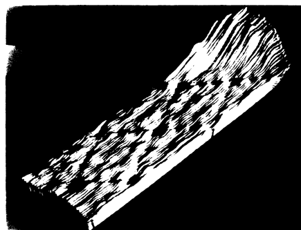
Three-dimensional model of a silicon surface made from two-dimensional scans by the STM. It shows two rhomboid-shaped unit cells. Hills and valleys within the cells, "never before observed" according to IBM, are less than 2.8 angstroms deep.
