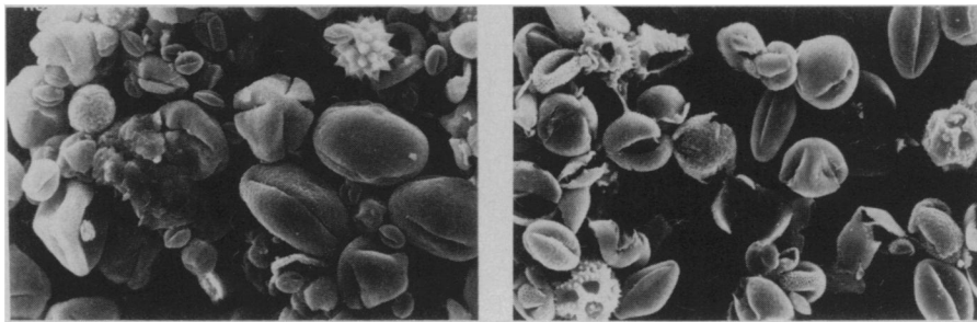
Electron microscope reveals that sample of yellow rain from an alleged attack (left) looks similar to bee excrement sample from Cambridge (right).
