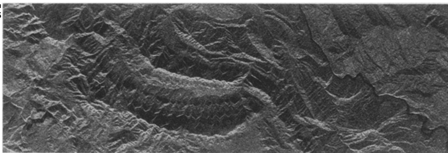
SIR-B radar image shows folded, layered rocks of the high plateau of northern Peru, crossed by the Marañon River, an Amazon tributary. Scene measures 14 by 42 km.
