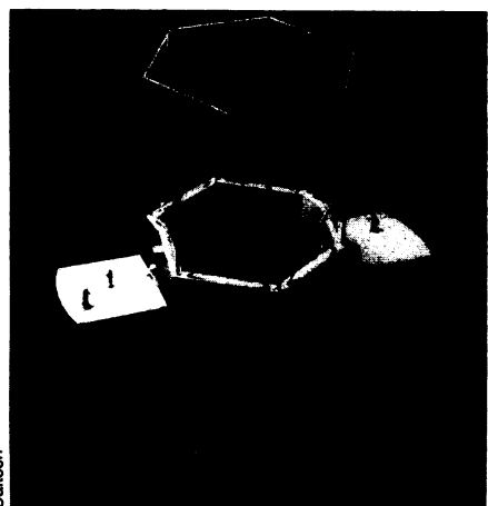
Model of the proposed 10-meter telescope shows the primary mirror built of hexagonal pieces and a secondary mirror hung at the top of the space frame, which will reflect rays back through a hole in the main mirror to a focus behind it.
