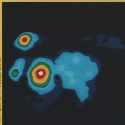
PET scan image of a horizontal "slice" through a breast cancer patient. Red-centered pattern (top) is the primary cancer. White-centered pattern is the liver, where the fluorine-18 estrogen analogue collects before being cleared from the body. The small green spot is a metastatic tumor in a lymph node.
