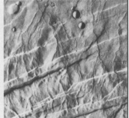
Viking photos of Mars show apparently fluid-formed channels not only on ancient, heavily cratered terrain (left) but also on a smoother region called Alba Patera (right), which may be as much as 2 billion years younger.
